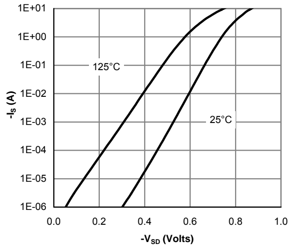
Figure 6: Body-Diode Characteristics
